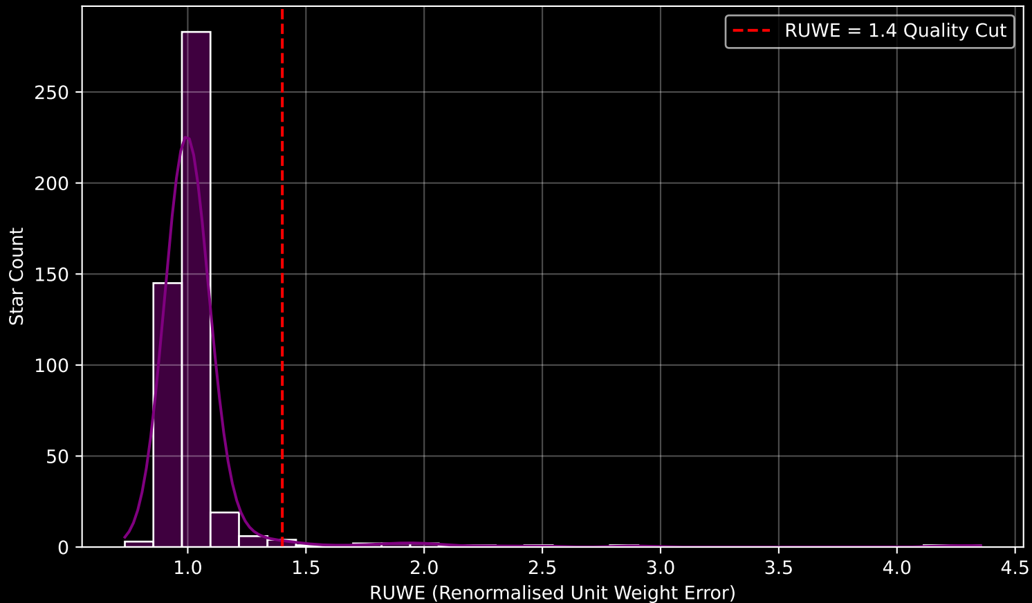
GAPOGEE DR17 Field [300-04] RUWE Distribution (n= 473)
