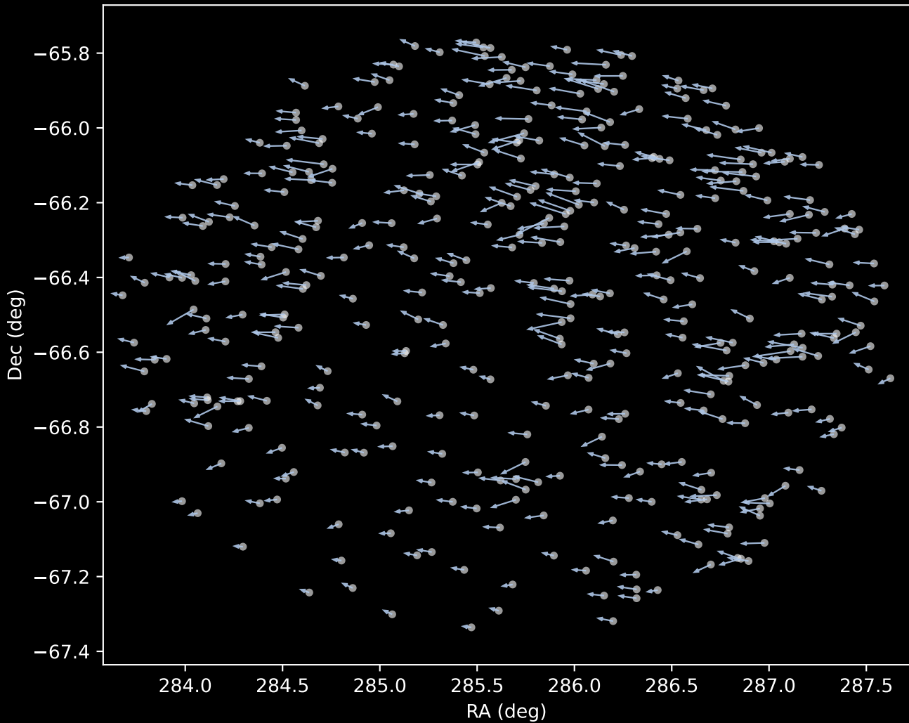
APOGEE DR17 Cluster 1 Proper Motion Vectors (n=399)
