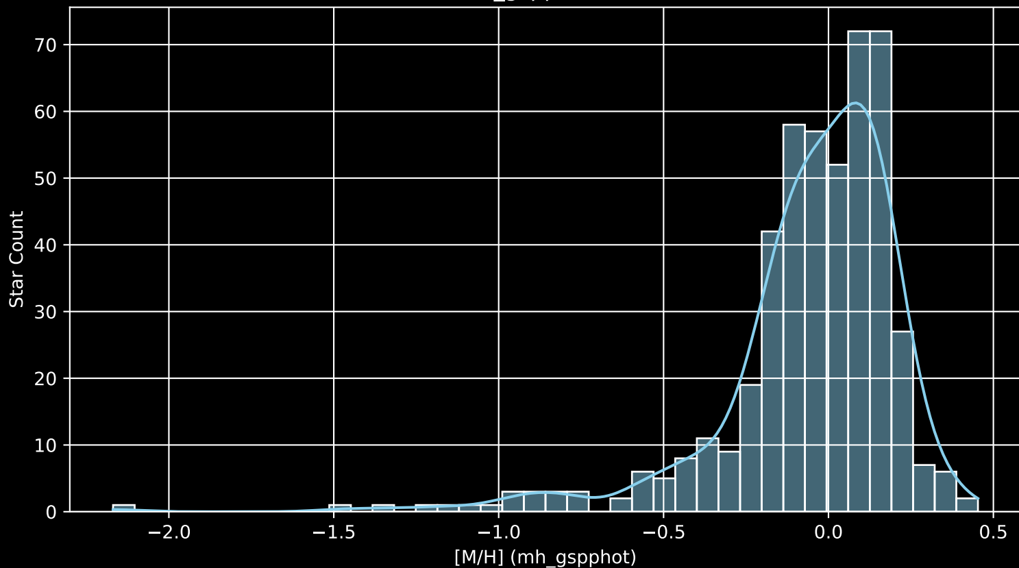
APOGEE DR17 Field: [300-04 [M/H] (mh_gspphot) (n= 474)
