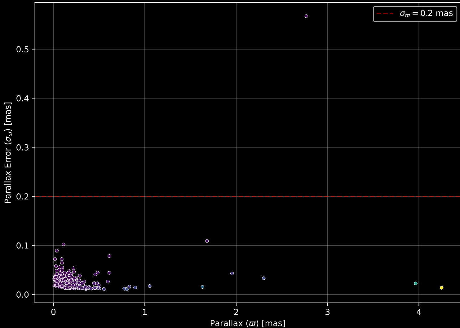
APOGEE DR17 Field: [300-04] Parallax Quality (n= 475)
