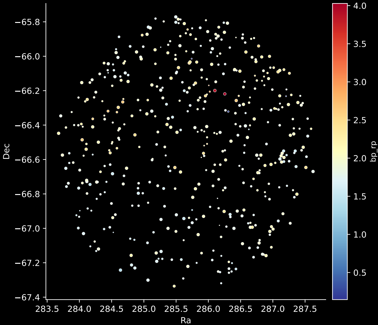
APOGEE DR17 Field: [300-04] Stars: 475
