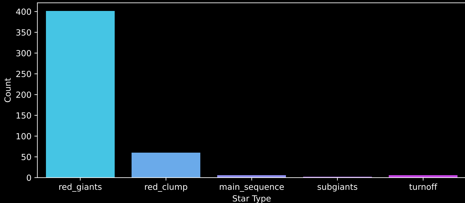
APOGEE DR17 Field: [300-04] Count plot of Star Type
