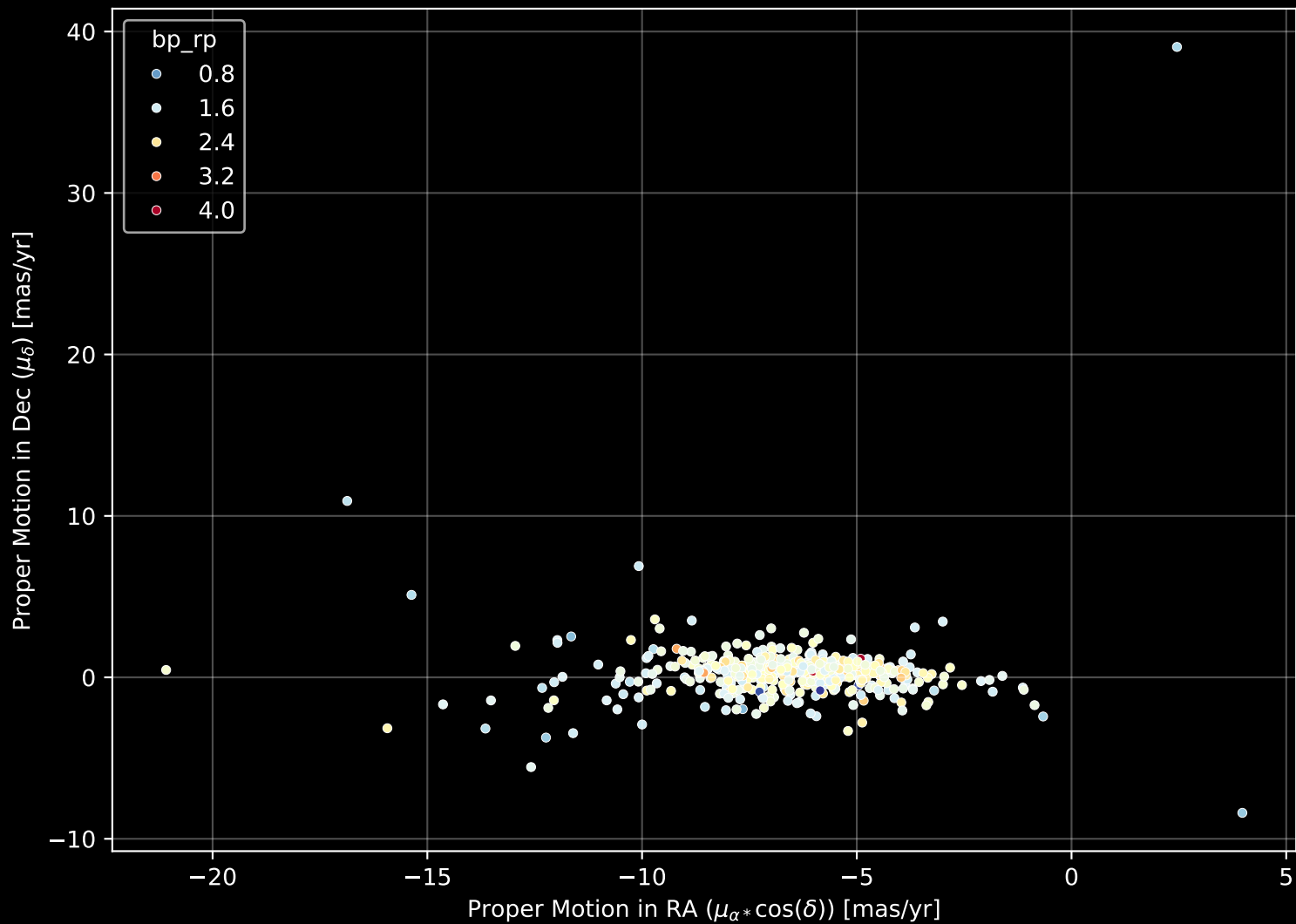
APOGEE DR17 Field: [300-04] Proper Motion Diagram (n= 475)
